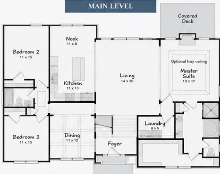
MAIN LEVEL
